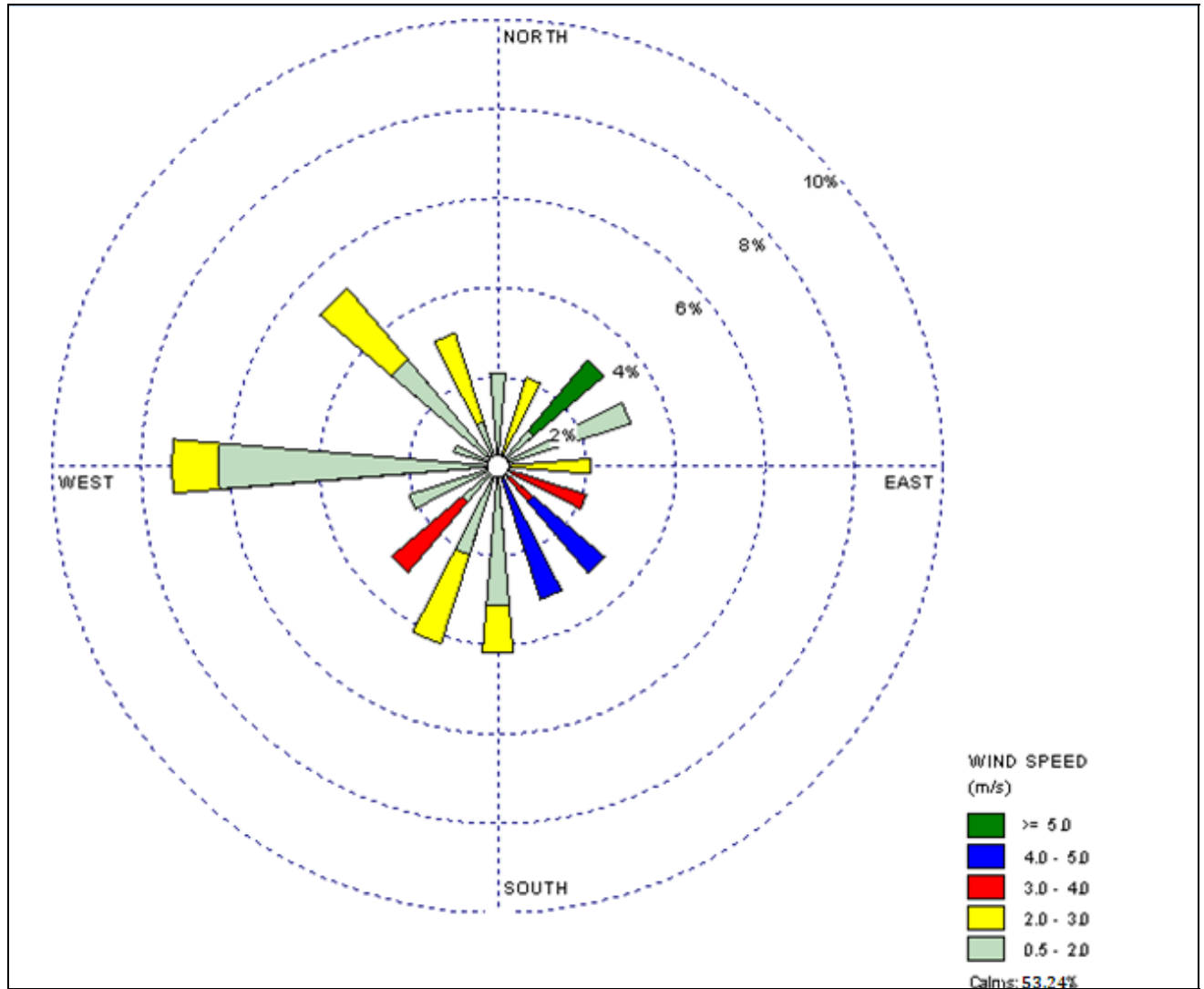
Figure- 3.1(a): WIND ROSE FOR MARCH 2009
