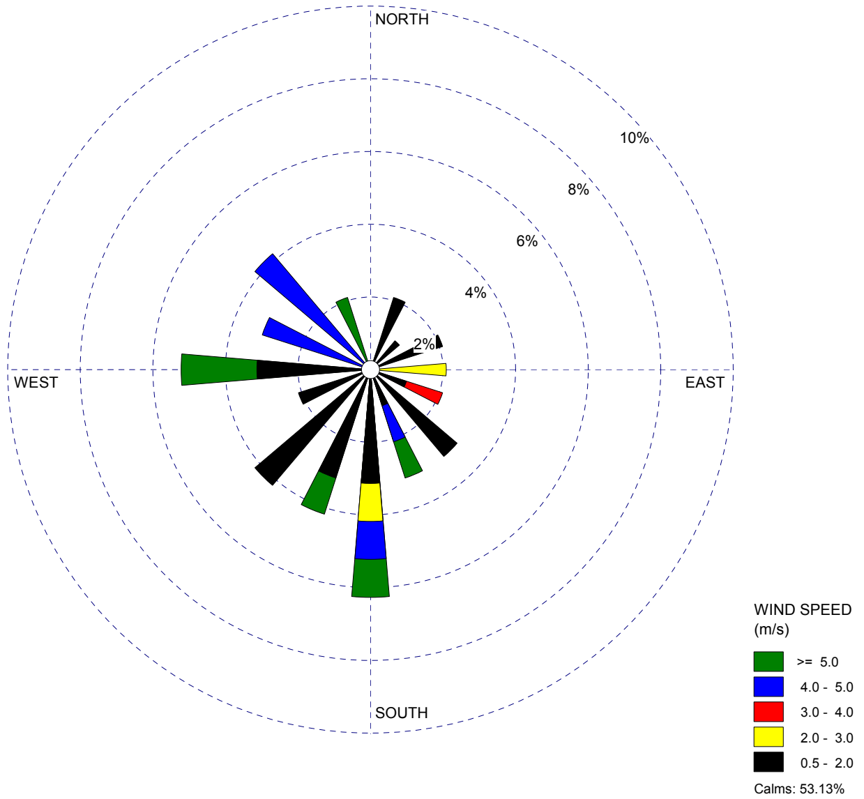
Figure- 3.1 (d): OVERALL WIND ROSE FOR SUMMER SEASON
