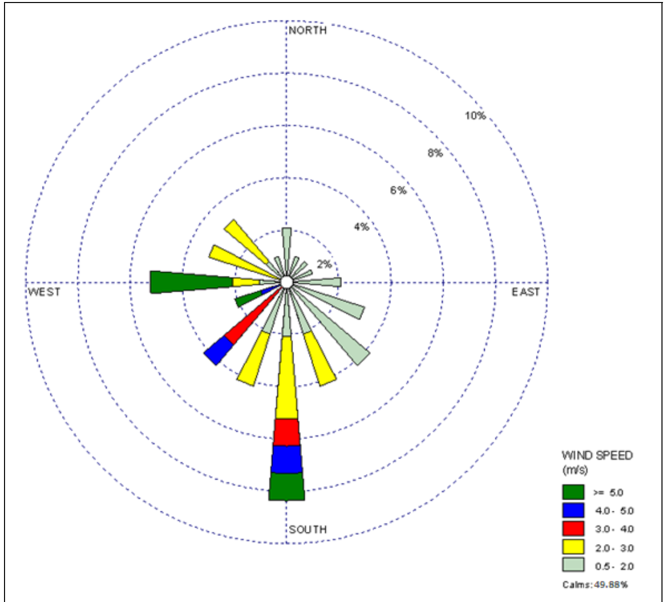
Figure- 3.1 (b): WIND ROSE FOR APRIL 2009
